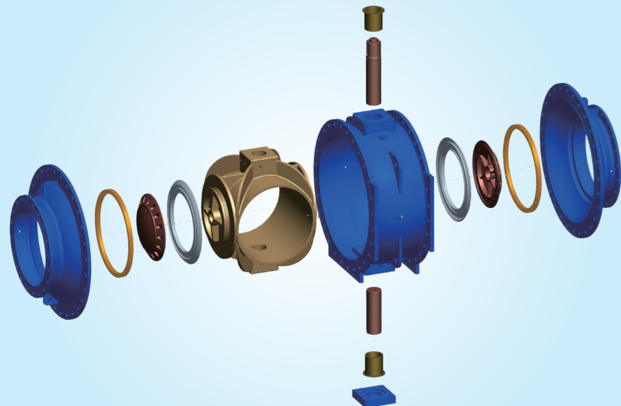
EXPLODED VIEW 分解圖
