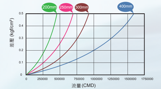
功能曲線圖 CHARACTERISTIC CURVE
