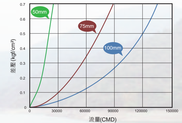
功能曲線圖 CHARACTERISTIC CURVE
