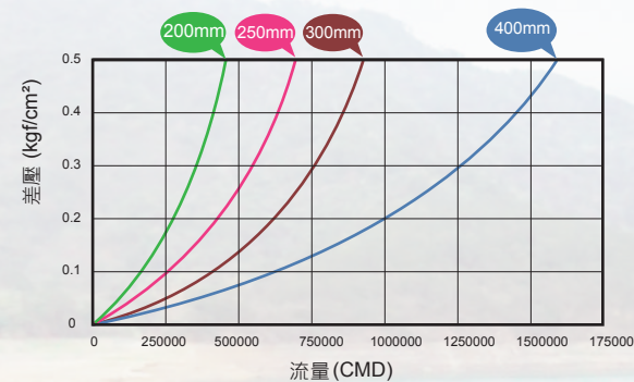
功能曲線圖 CHARACTERISTIC CURVE
